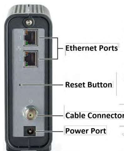
Figure 2: CM8200 Rear View
